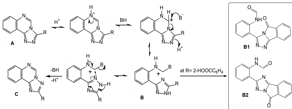
Fig. 2. Dimroth rearrangement associated side product formation
